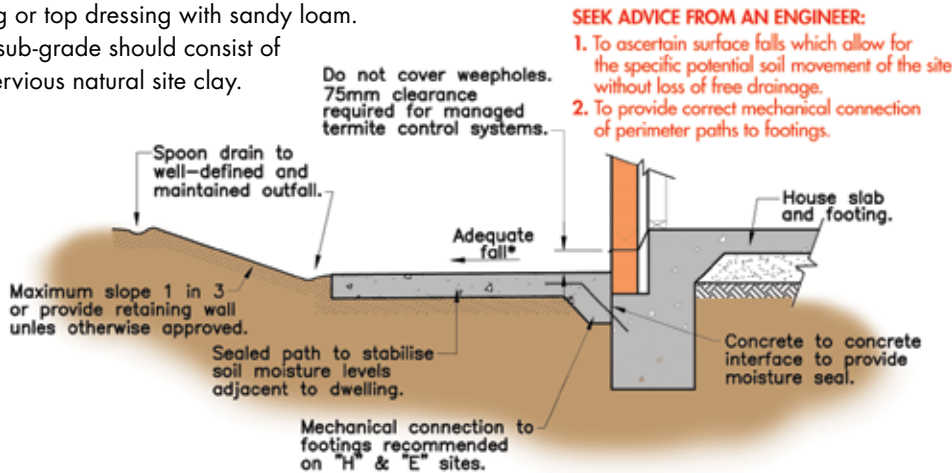
RECOMMENDED DRAINAGE AND MAINTENANCE ADJACENT TO DWELLING
